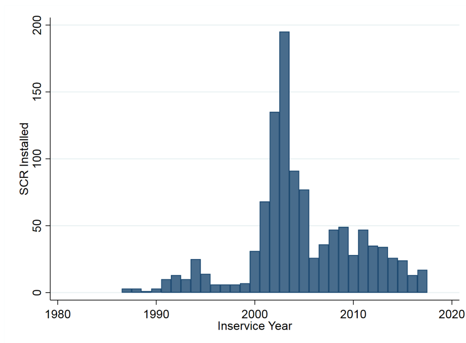
Figure B-7: Installation of Selective Catalytic Reduction (SCR)
