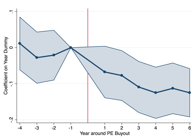
Panel A: Instruction Spending Share Event Study (Regression Coefficients by Year)
