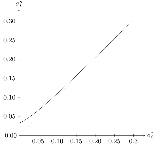
Figure 7: This Figure illustrates the link between fundamental volatility \sigma_i^r in an economy with traditional agents, and volatility \sigma_i^s in an economy with sparse agents (solid line). The dashed line is the 45 degree line. Parameters: \alpha = 1 , \frac{\psi_i c_i^d p_i^d}{\kappa} = 10^3 .
