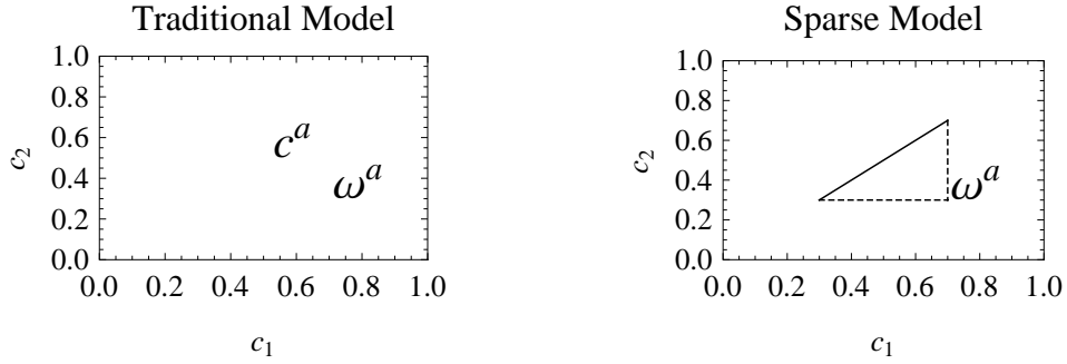
Figure 6: These Edgeworth boxes show competitive equilibria when both agents have Leontief preferences. The left panel illustrates the traditional model with rational agents: there is just one equilibrium, c^a = (1/2, 1/2) . The right panel illustrates the situation when type a is rational, and type b is boundedly rational: there is a one-dimensional continuum of competitive equilibria. Agent a 's share of the total endowment ( \omega^a ) is the same in both cases.
