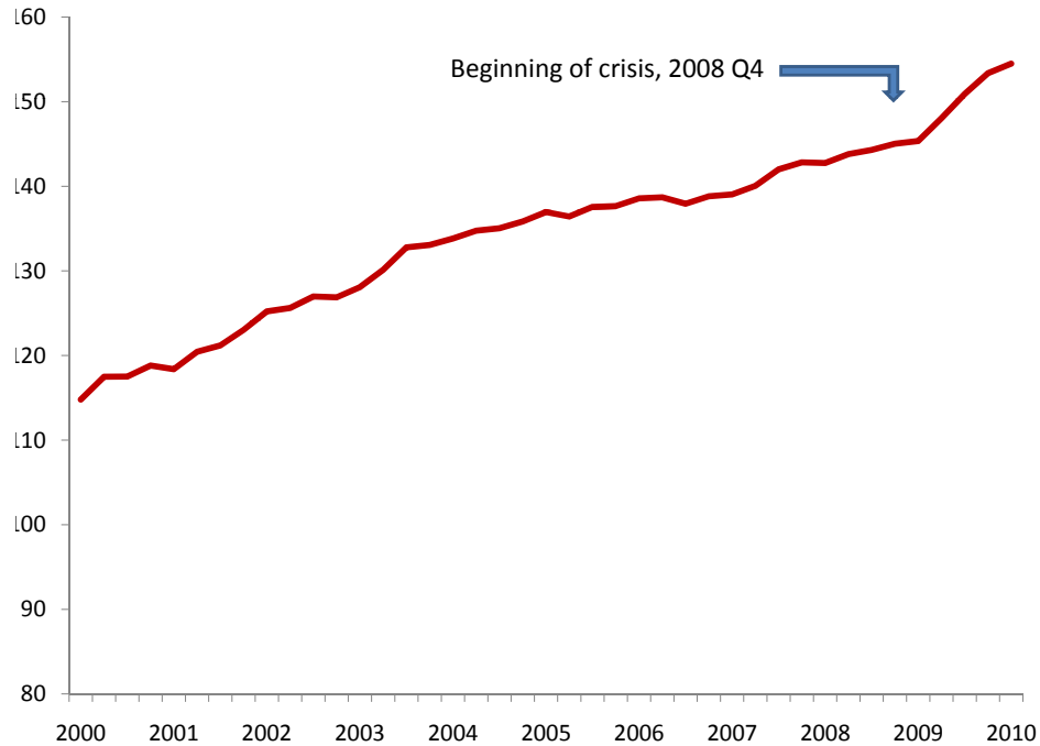
Figure 4: Index of Output per Hour, Total U.S. Economy
