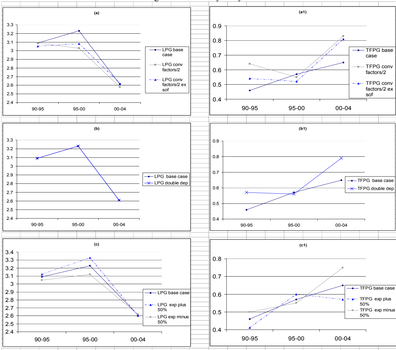
Figure 4: Sensitivity analysis
